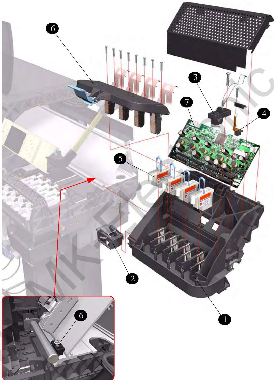
Figure 8: Carriage Assembly
